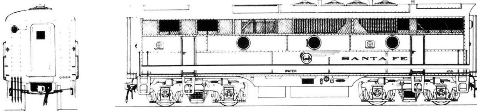
B-UNITS NAME TOWARDS REAR ON BOTH SIDES, UNIT NUMBERS TOWARD REAR BOTH SIDES. INDIAN FACES FRONT BOTH SIDES.
