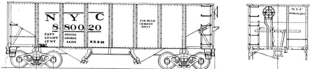
NEW YORK CENTRAL 34FT ASRA 2 BAY HOPPER: Paint entire car reefer grey. Lettering is black.
